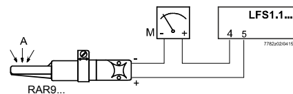
Photocell detector RAR9
