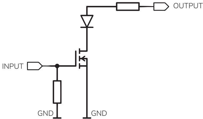
Functional diagram passive output
