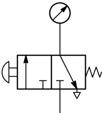
Fig. 3: Switching scheme
