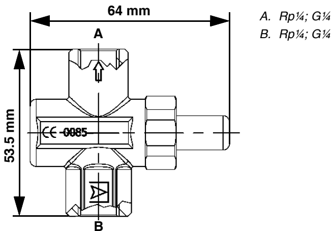
Fig. 2: Dimensions and connections ( Rp\frac{1}{4} ; G\frac{1}{4} )
