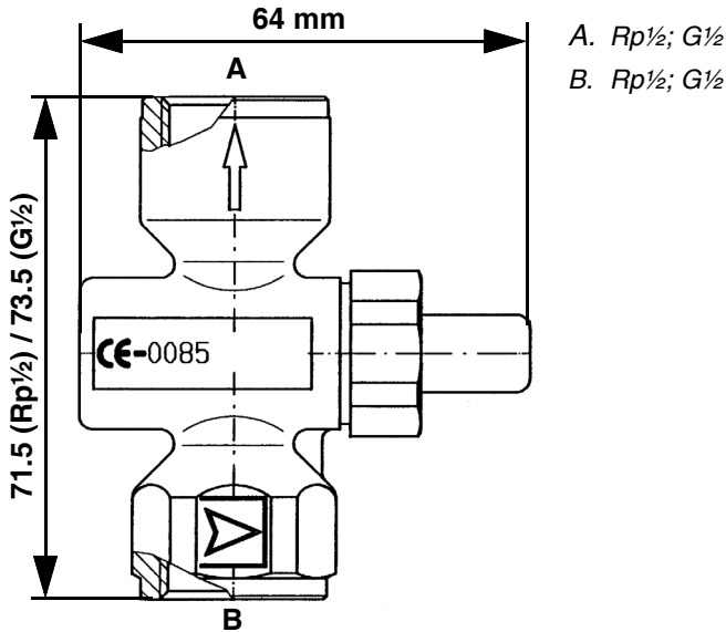
Fig. 1: Dimensions and connections ( Rp\frac{1}{2} ; G\frac{1}{2} )
